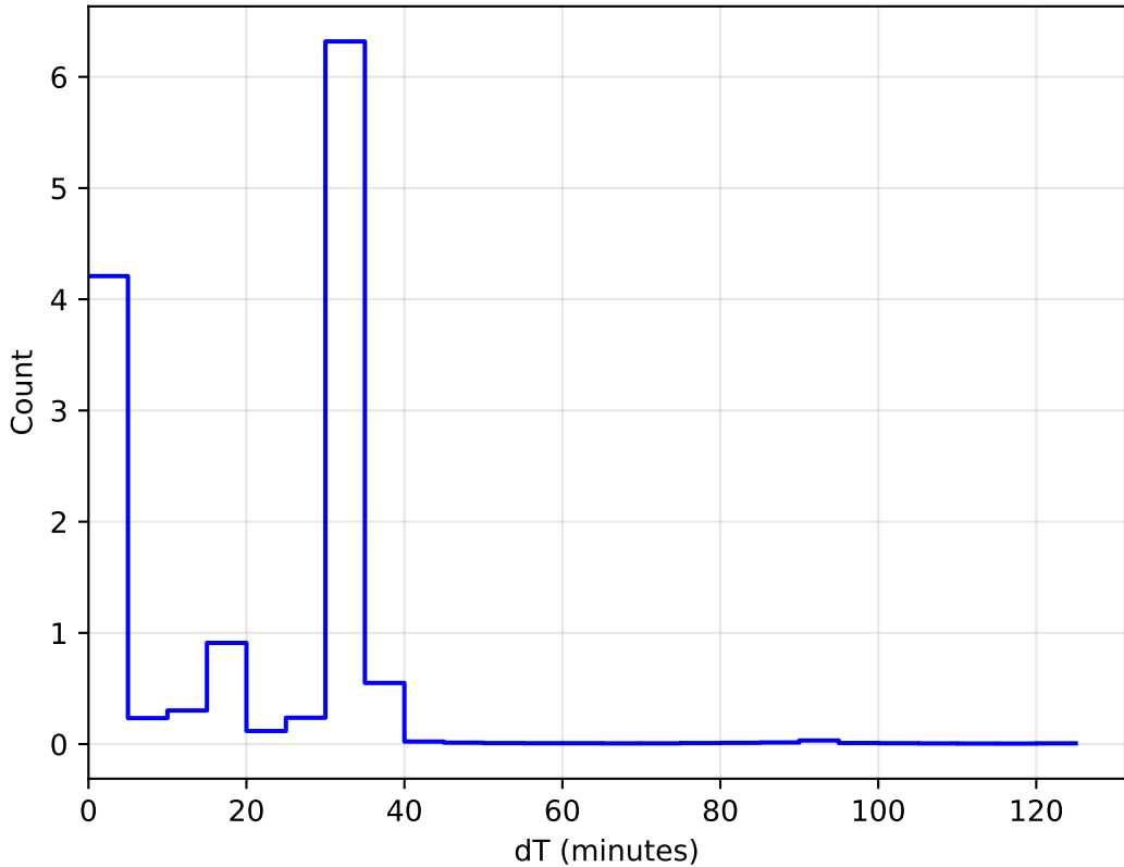
ddf_acor_sf30_lsf40_lsr10_v3.4_10yrs All sky: DeltaT Histogram
