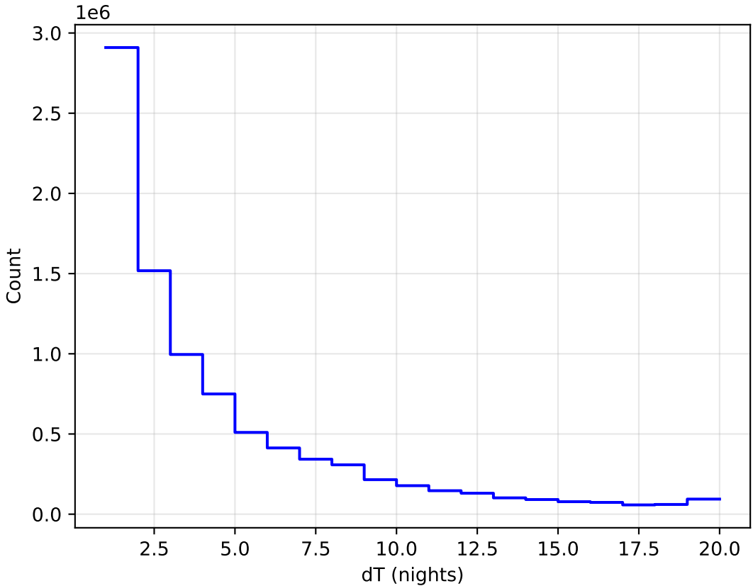
ddf_acor_sf30_lsf40_lsr10_v3.4_10yrs All sky all bands: DeltaNight Histogram
