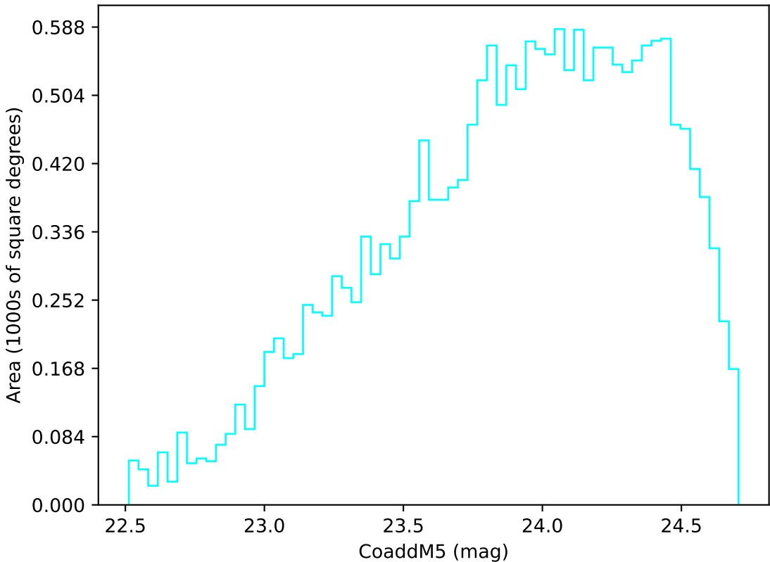
ddf_acor_sf30_lsf40_lsr10_v3.4_10yrs Yr 3-4 u band: CoaddM5
