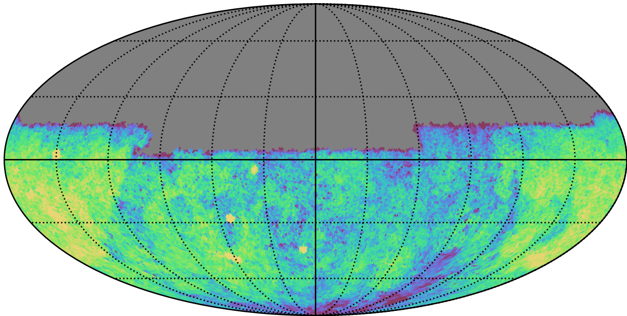
ddf_acor_sf30_lsf40_lsr10_v3.4_10yrs Yr 1 u band: CoaddM5
