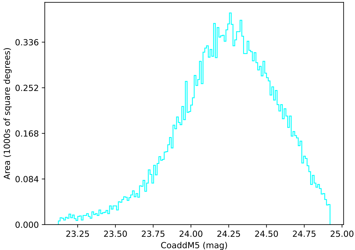
ddf_acor_sf30_lsf40_lsr10_v3.4_10yrs Yr 1 u band: CoaddM5
