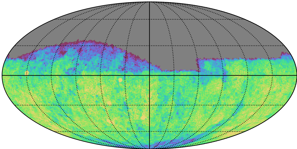
ddf_acor_sf30_lsf40_lsr10_v3.4_10yrs Yr 1 g band: CoaddM5
