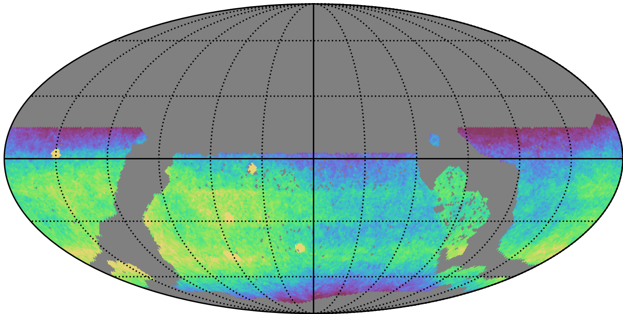
ddf_acor_sf30_lsf40_lsr10_v3.4_10yrs WFD r band: CoaddM5
