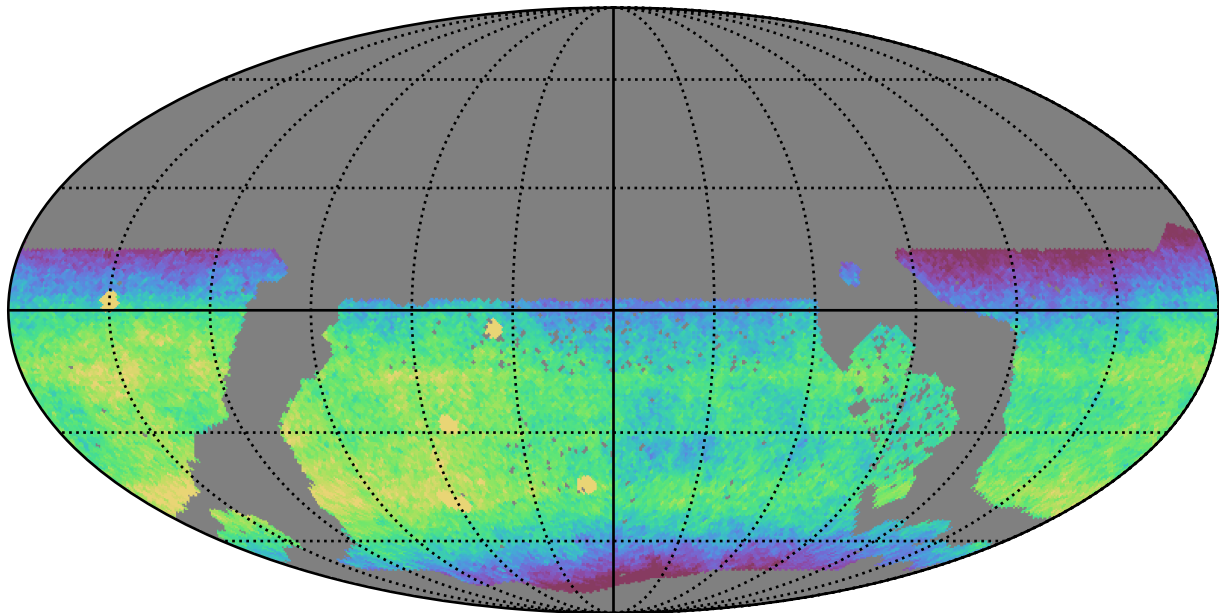
ddf_acor_sf30_lsf40_lsr10_v3.4_10yrs WFD i band: CoaddM5
