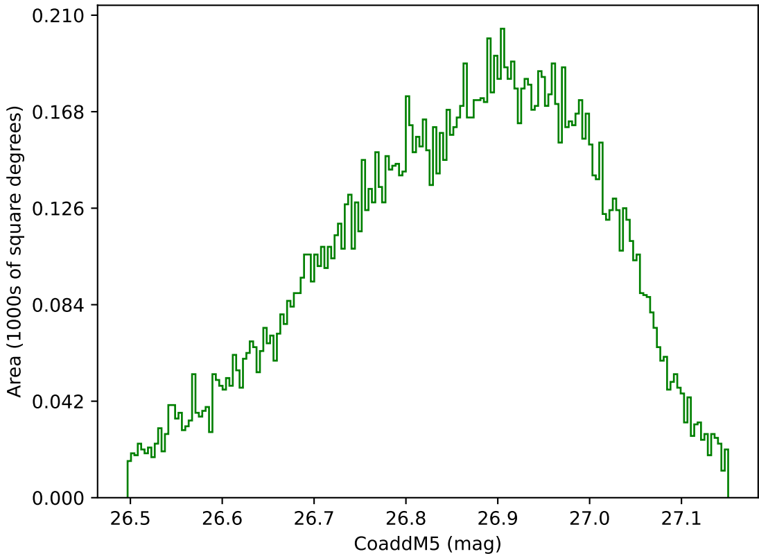
ddf_acor_sf30_lsf40_lsr10_v3.4_10yrs WFD g band: CoaddM5
