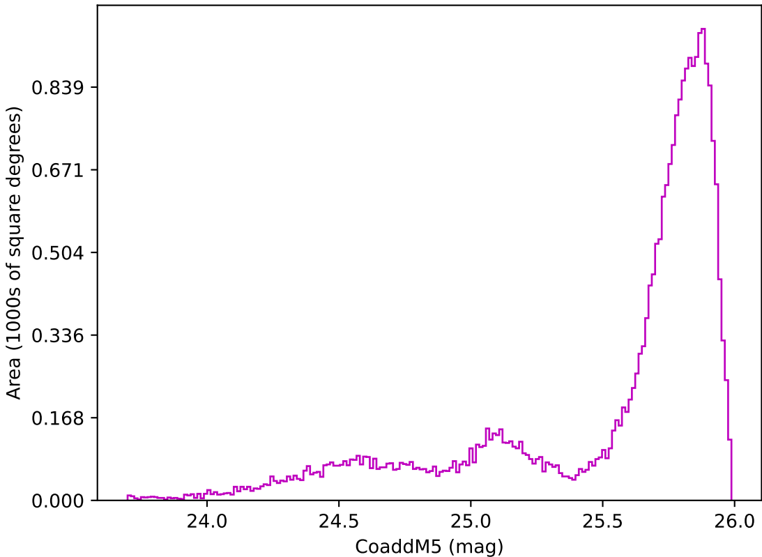
ddf_acor_sf30_lsf40_lsr10_v3.4_10yrs All sky z band: CoaddM5
