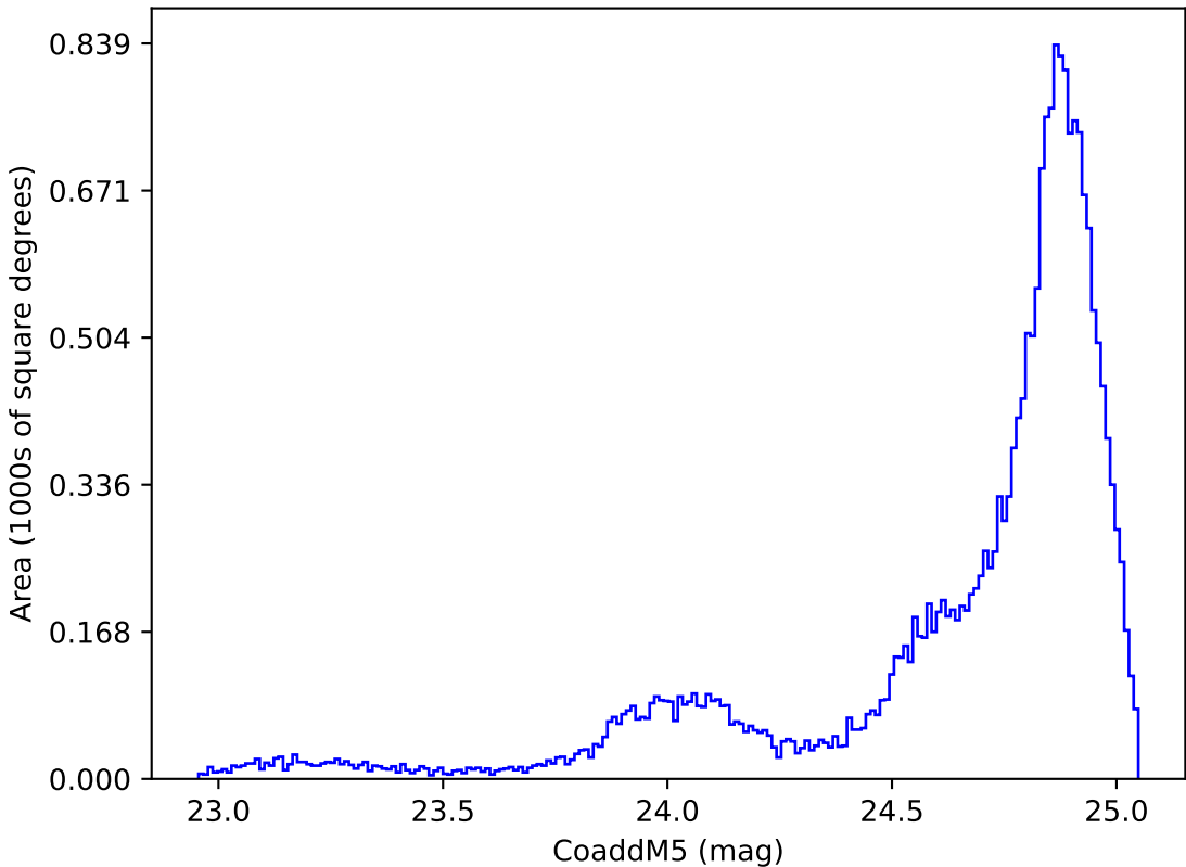
ddf_acor_sf30_lsf40_lsr10_v3.4_10yrs All sky y band: CoaddM5
