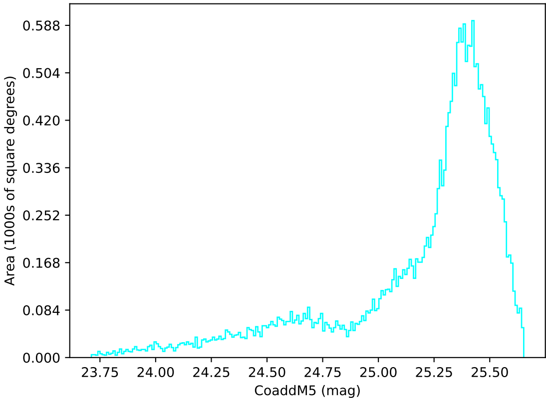
ddf_acor_sf30_lsf40_lsr10_v3.4_10yrs All sky u band: CoaddM5
