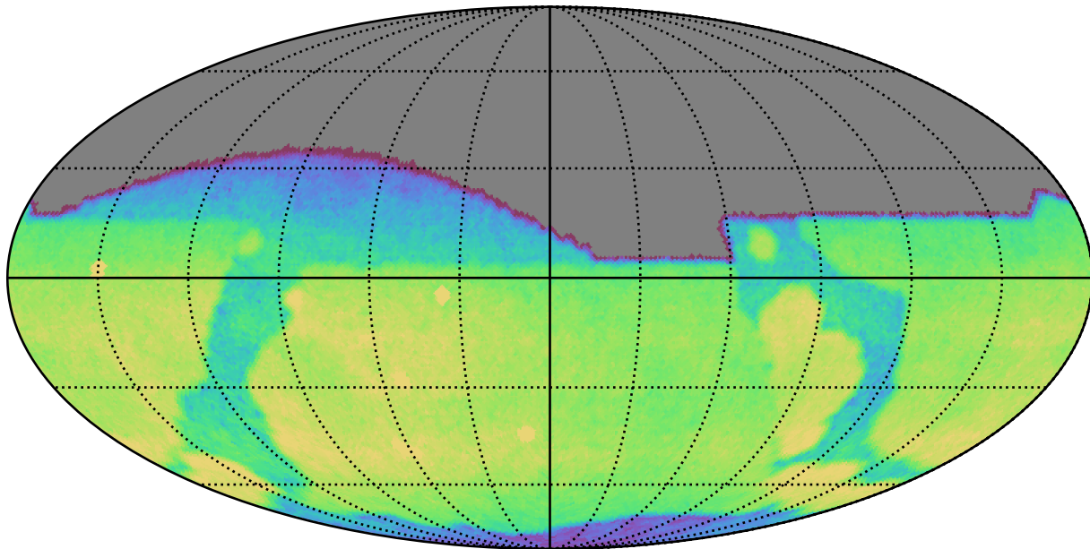
ddf_acor_sf30_lsf40_lsr10_v3.4_10yrs All sky g band: CoaddM5
