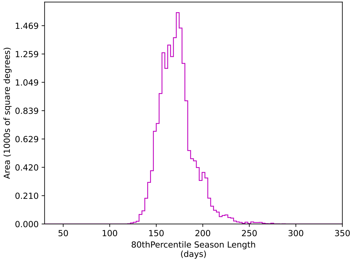
ddf_acor_sf30_lsf40_lsr10_v3.4_10yrs WFD z band: 80thPercentile Season Length
