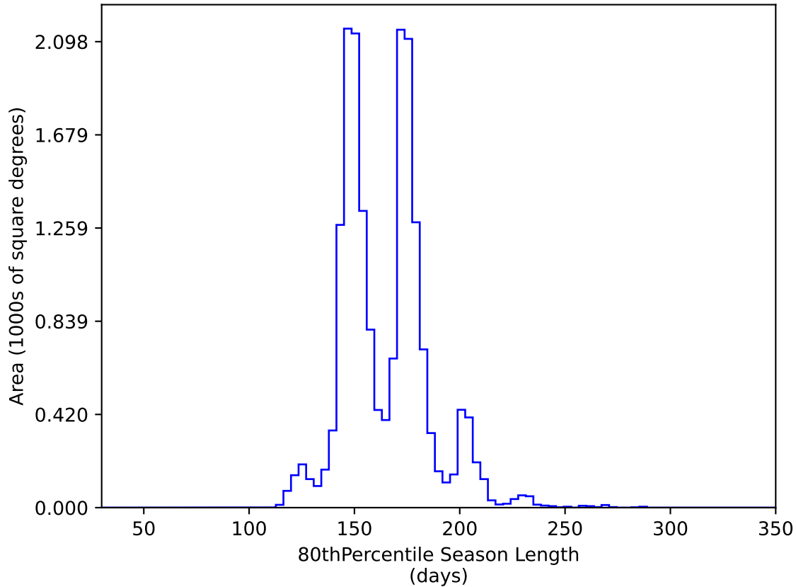
ddf_acor_sf30_lsf40_lsr10_v3.4_10yrs WFD y band: 80thPercentile Season Length
