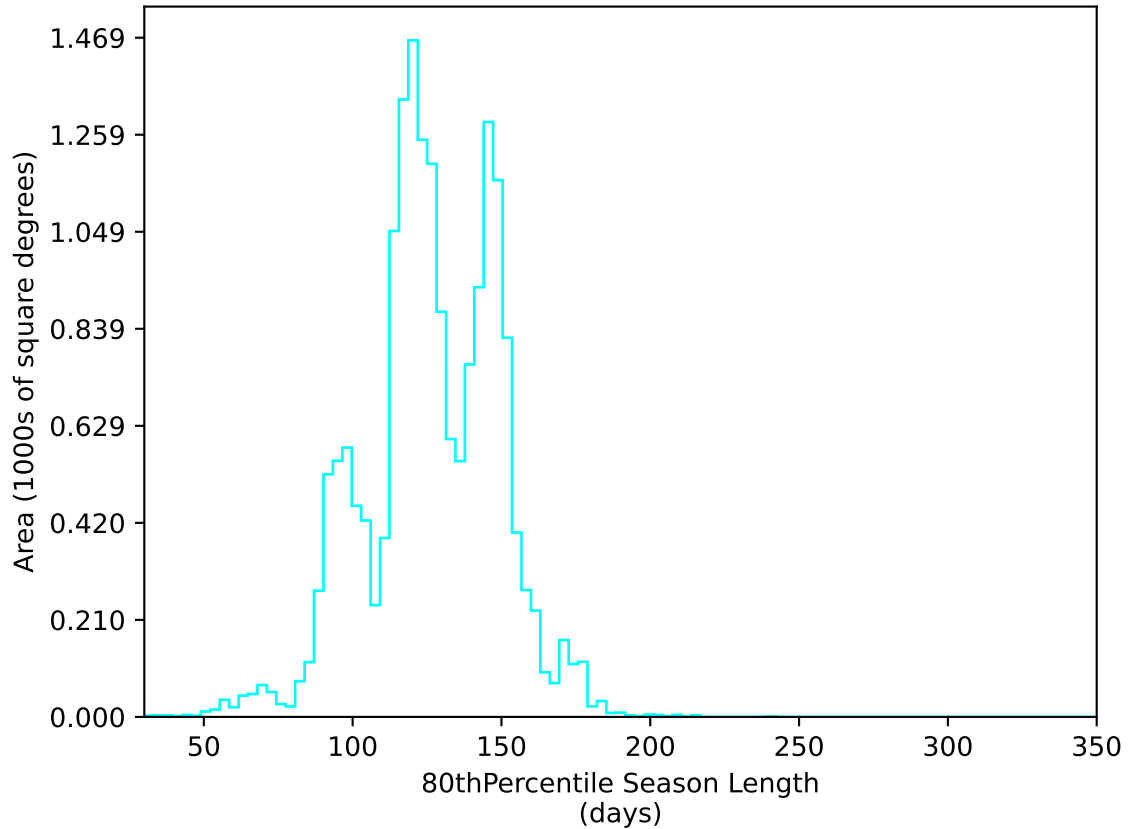
ddf_acor_sf30_lsf40_lsr10_v3.4_10yrs WFD u band: 80thPercentile Season Length
