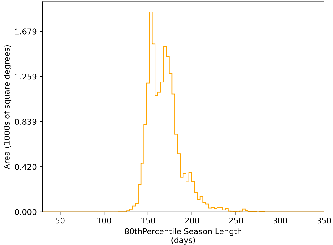
ddf_acor_sf30_lsf40_lsr10_v3.4_10yrs WFD r band: 80thPercentile Season Length
