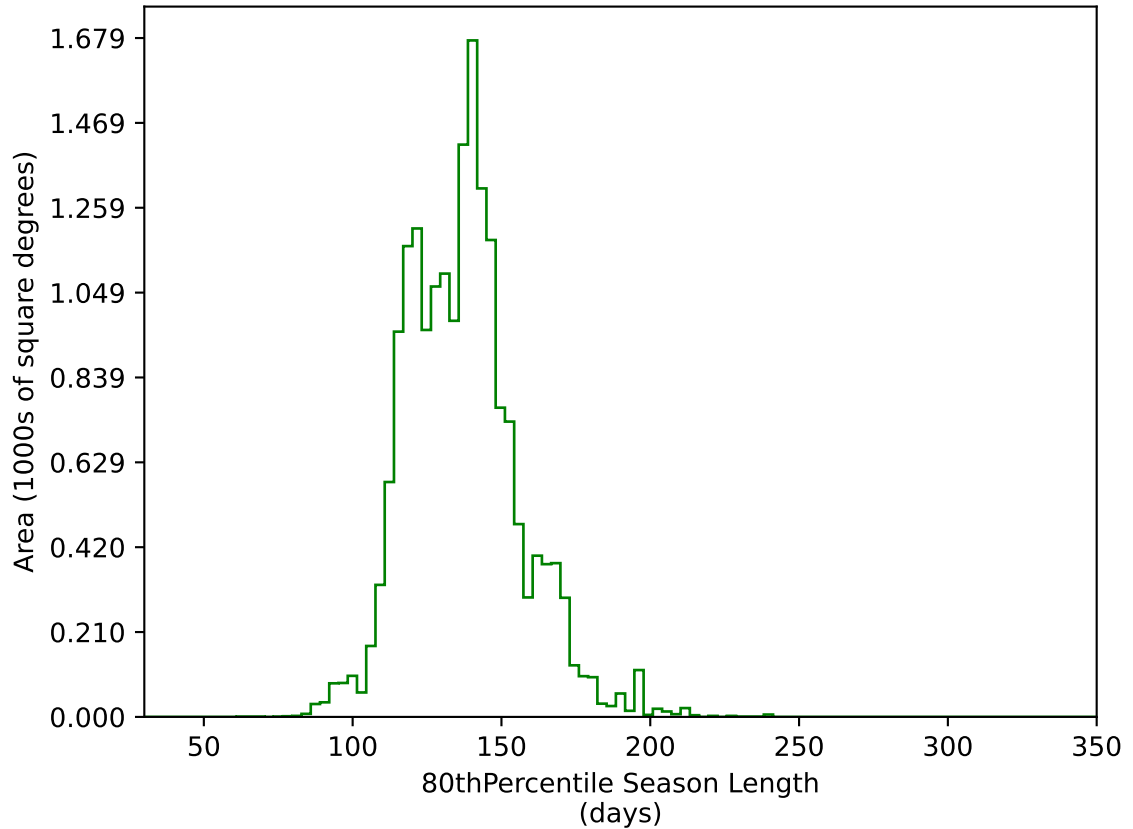
ddf_acor_sf30_lsf40_lsr10_v3.4_10yrs WFD g band: 80thPercentile Season Length
