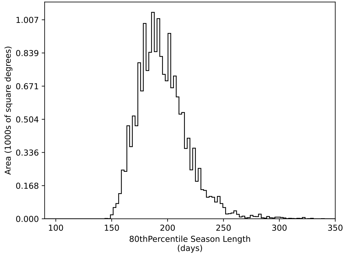
ddf_acor_sf30_lsf40_lsr10_v3.4_10yrs WFD all bands: 80thPercentile Season Length
