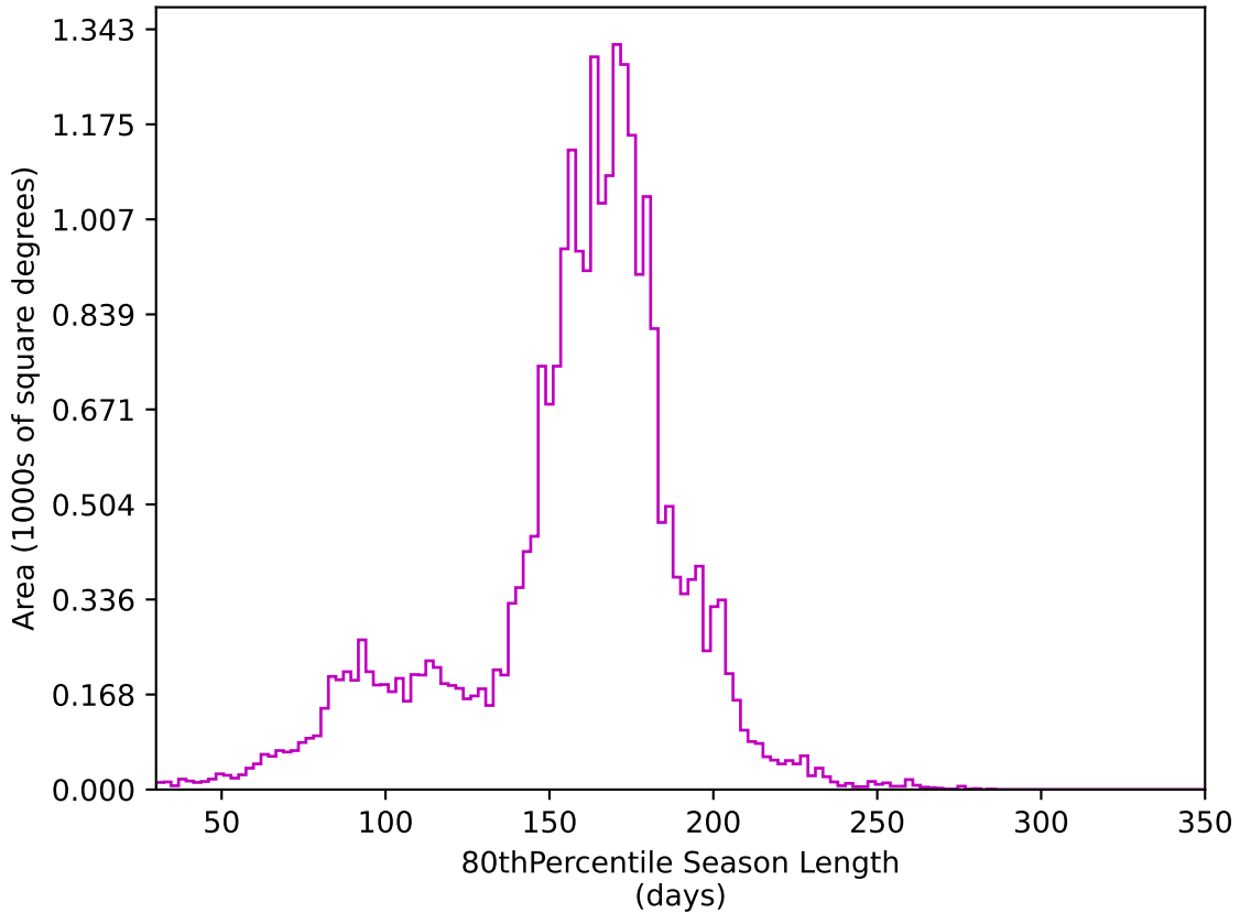
ddf_acor_sf30_lsf40_lsr10_v3.4_10yrs All sky z band: 80thPercentile Season Length
