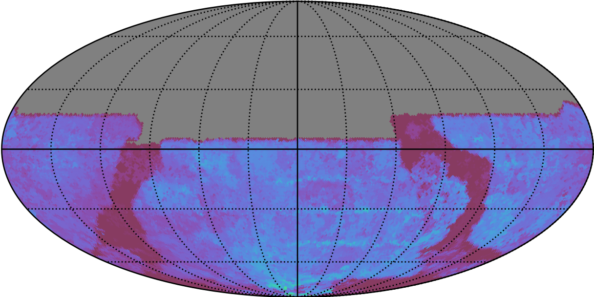
ddf_acor_sf30_lsf40_lsr10_v3.4_10yrs All sky u band: 80thPercentile Season Length
