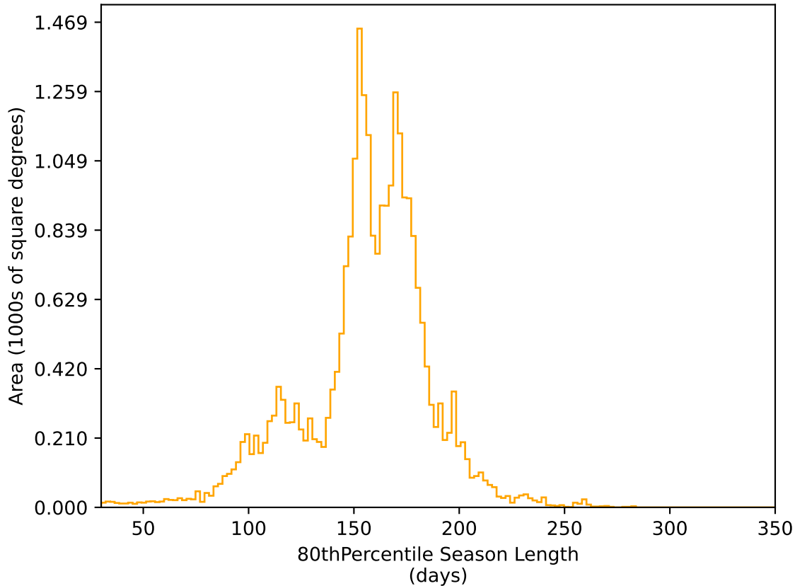
ddf_acor_sf30_lsf40_lsr10_v3.4_10yrs All sky r band: 80thPercentile Season Length
