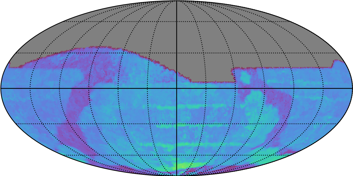
ddf_acor_sf30_lsf40_lsr10_v3.4_10yrs All sky i band: 80thPercentile Season Length
