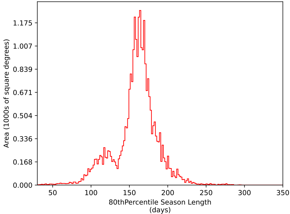
ddf_acor_sf30_lsf40_lsr10_v3.4_10yrs All sky i band: 80thPercentile Season Length
