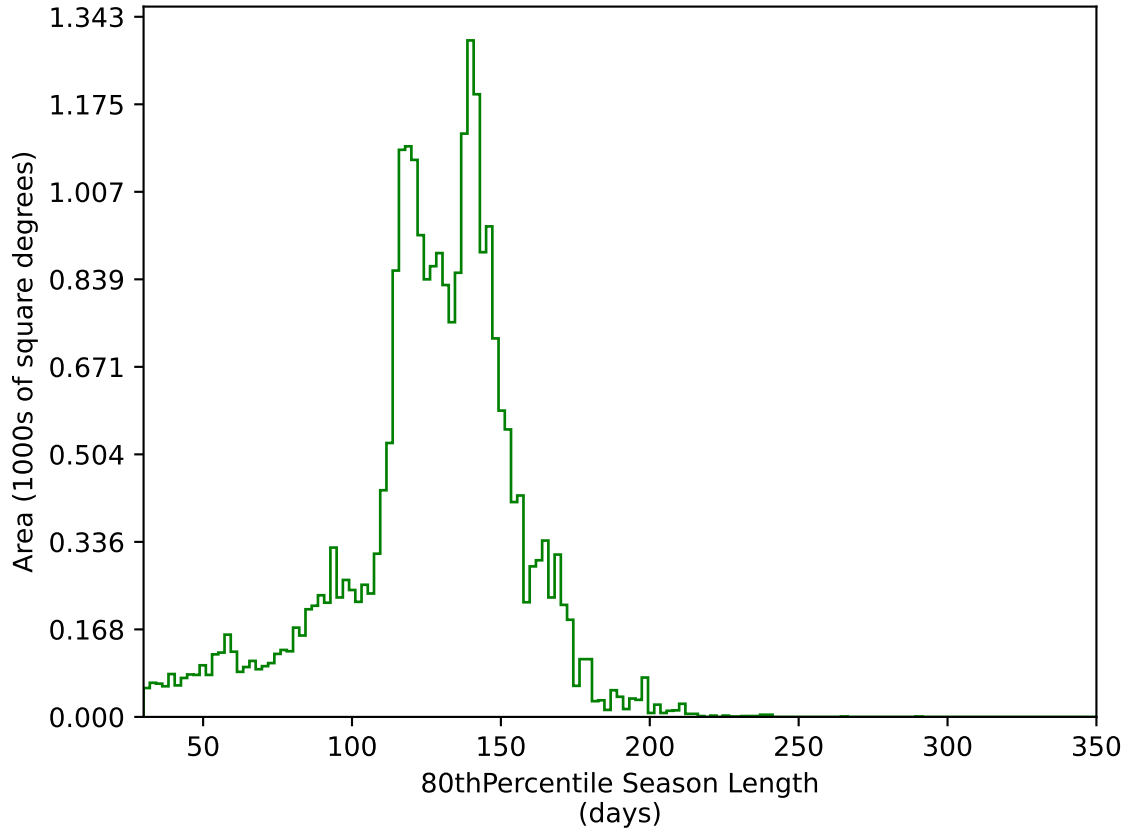
ddf_acor_sf30_lsf40_lsr10_v3.4_10yrs All sky g band: 80thPercentile Season Length
