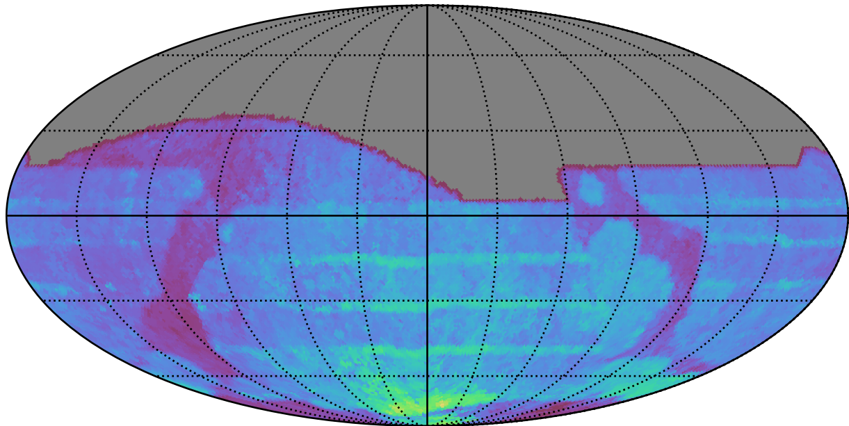
ddf_acor_sf30_lsf40_lsr10_v3.4_10yrs All sky all bands: 80thPercentile Season Length
