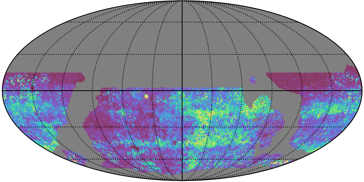
ddf_acor_sf30_lsf40_lsr10_v3.4_10yrs WFD zy bands: 75th Percentile Intranight Timespan
