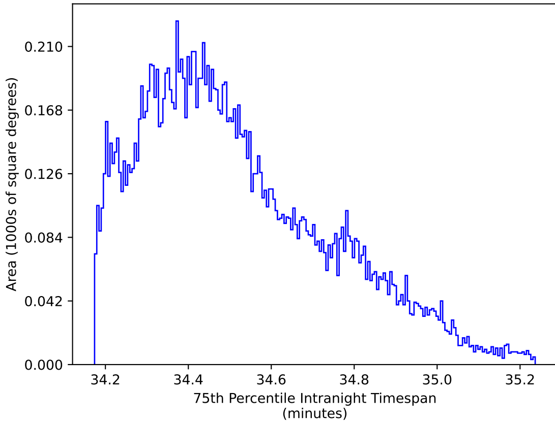
ddf_acor_sf30_lsf40_lsr10_v3.4_10yrs WFD zy bands: 75th Percentile Intranight Timespan
