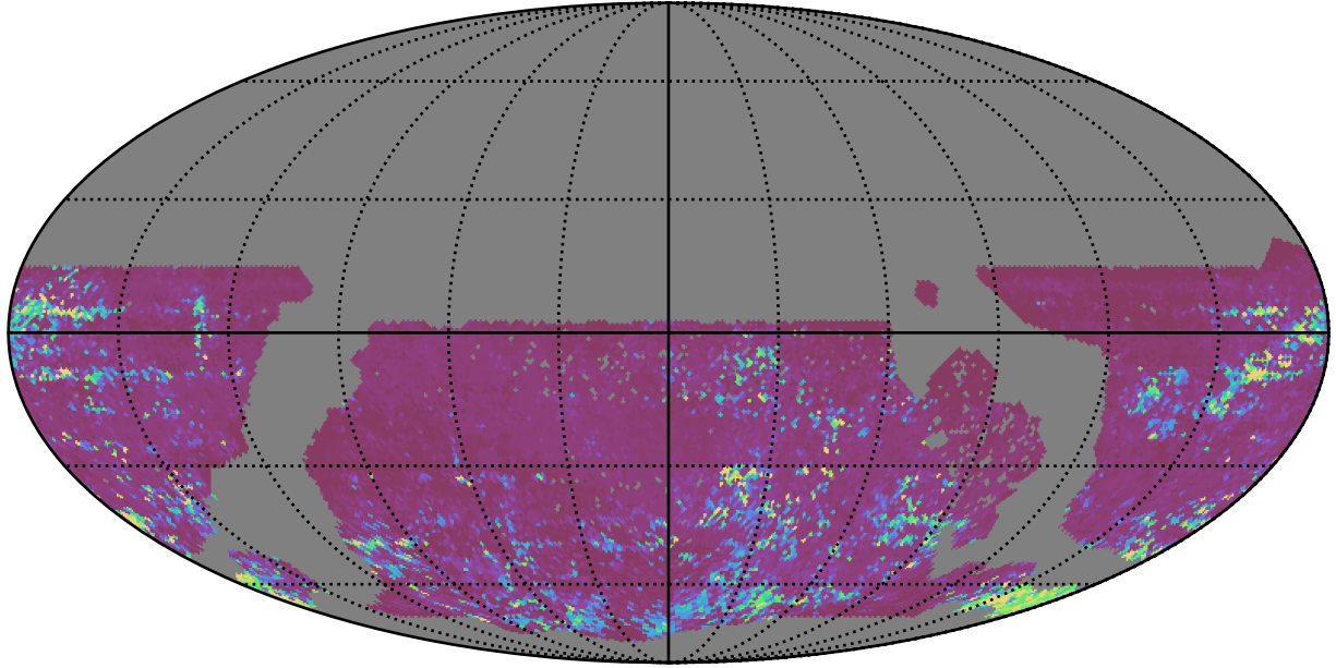
ddf_acor_sf30_lsf40_lsr10_v3.4_10yrs WFD z band: 75th Percentile Intranight Timespan
