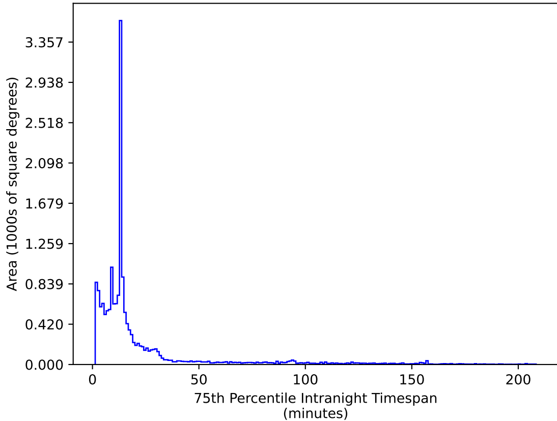
ddf_acor_sf30_lsf40_lsr10_v3.4_10yrs WFD z band: 75th Percentile Intranight Timespan
