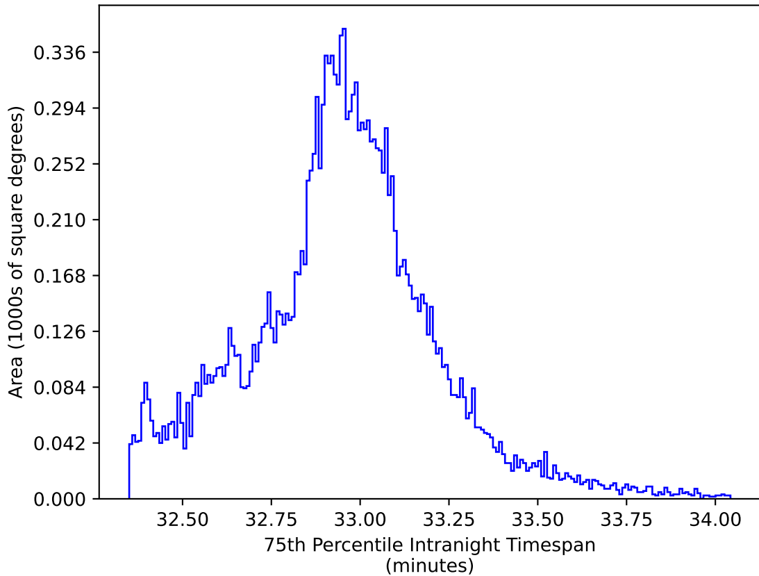
ddf_acor_sf30_lsf40_lsr10_v3.4_10yrs WFD y band: 75th Percentile Intranight Timespan
