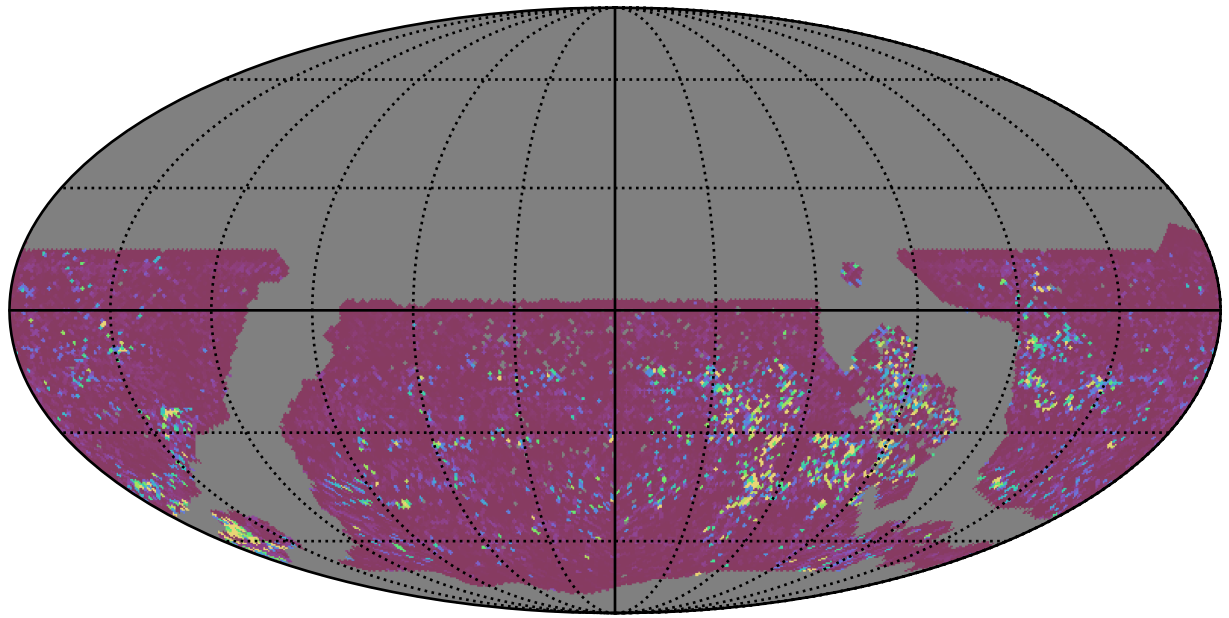
ddf_acor_sf30_lsf40_lsr10_v3.4_10yrs WFD u band: 75th Percentile Intranight Timespan
