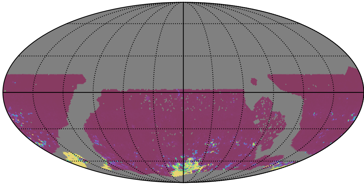
ddf_acor_sf30_lsf40_lsr10_v3.4_10yrs WFD ri bands: 75th Percentile Intranight Timespan
