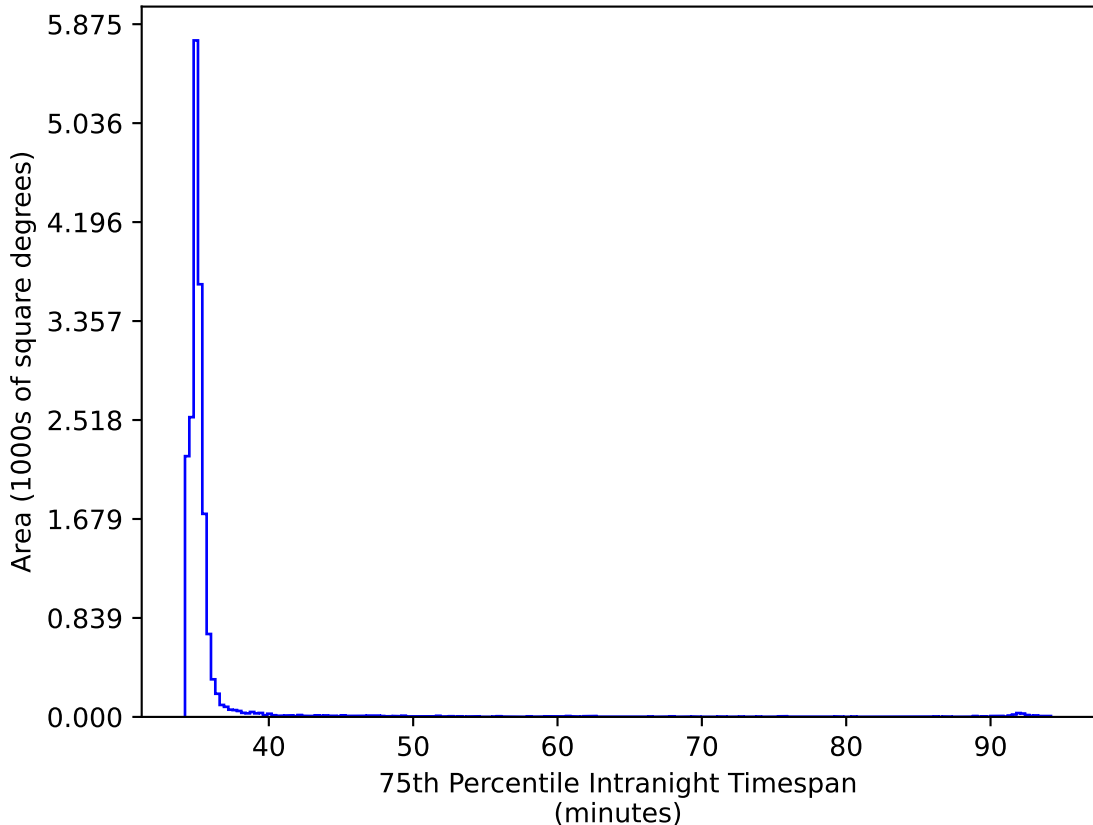
ddf_acor_sf30_lsf40_lsr10_v3.4_10yrs WFD ri bands: 75th Percentile Intranight Timespan
