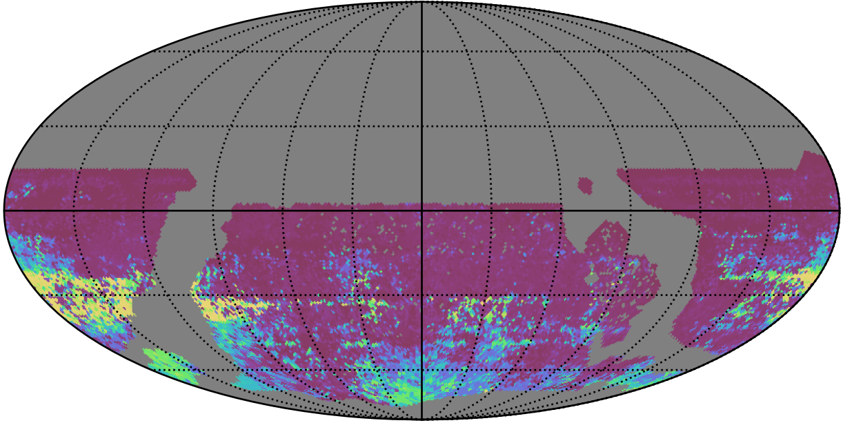
ddf_acor_sf30_lsf40_lsr10_v3.4_10yrs WFD r band: 75th Percentile Intranight Timespan
