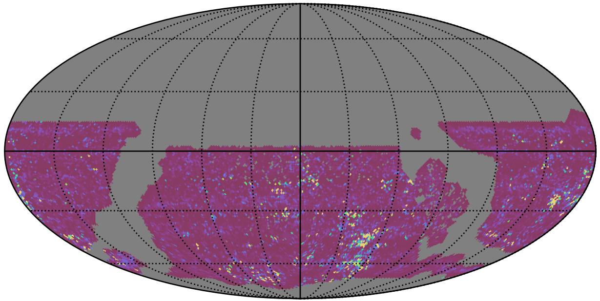
ddf_acor_sf30_lsf40_lsr10_v3.4_10yrs WFD g band: 75th Percentile Intranight Timespan
