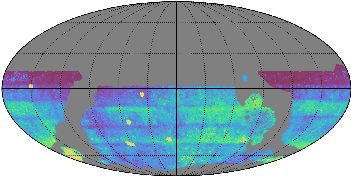
ddf_acor_sf30_ls40_lsr10_v3.4_10yrs WFD: 75th Percentile Intranight Timespan
