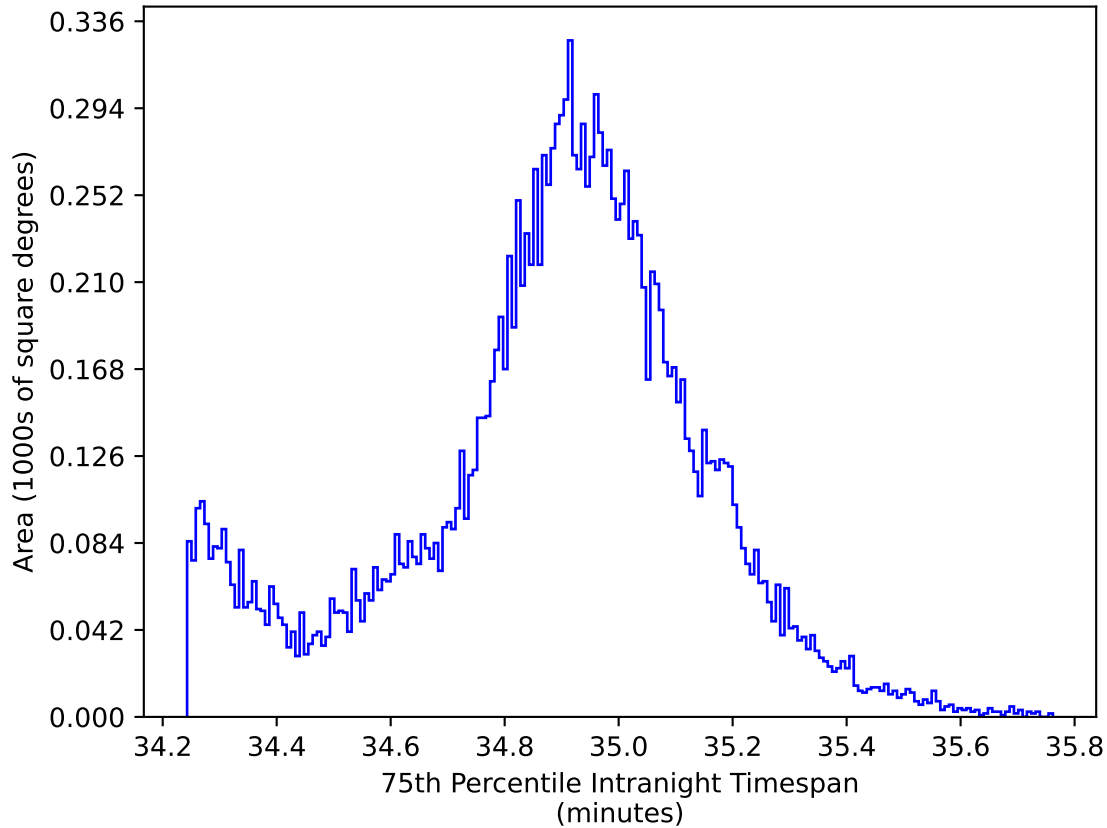
ddf_acor_sf30_lsf40_lsr10_v3.4_10yrs WFD: 75th Percentile Intranight Timespan
