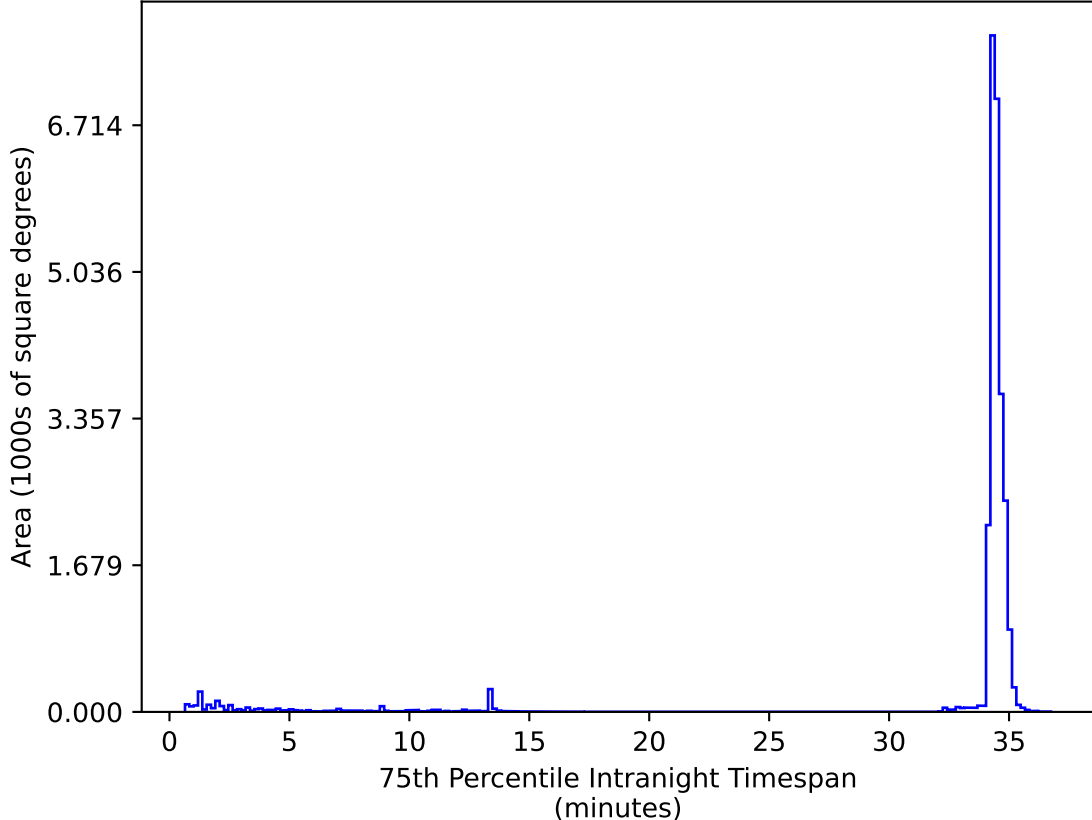
ddf_acor_sf30_lsf40_lsr10_v3.4_10yrs All sky zy bands: 75th Percentile Intranight Timespan
