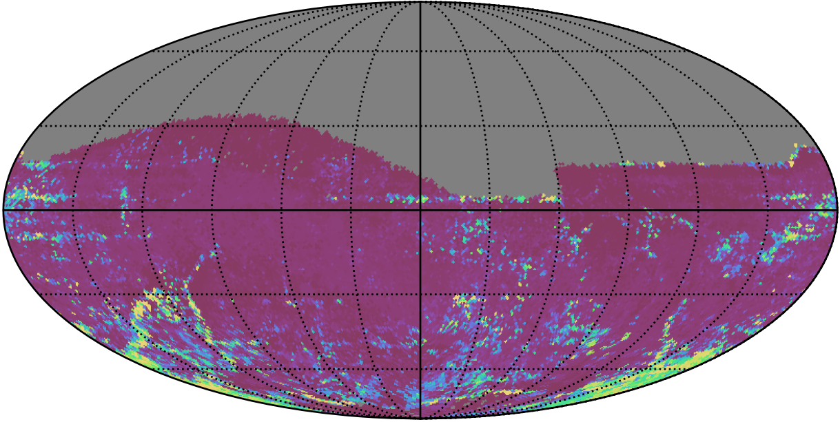
ddf_acor_sf30_lsf40_lsr10_v3.4_10yrs All sky z band: 75th Percentile Intranight Timespan
