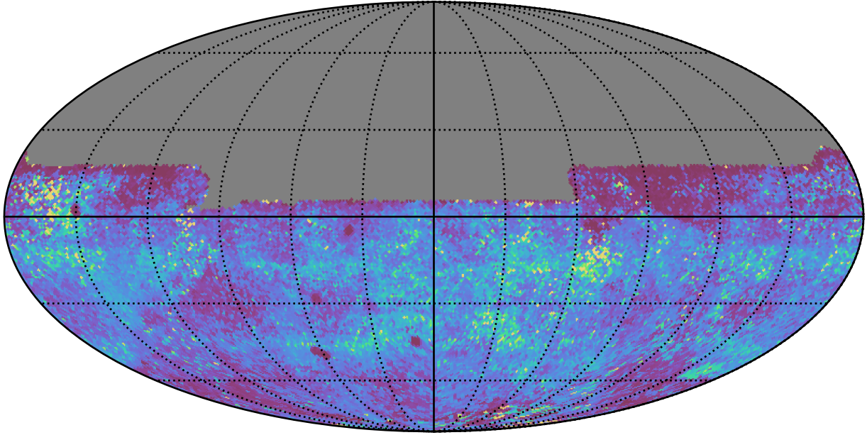
ddf_acor_sf30_lsf40_lsr10_v3.4_10yrs All sky y band: 75th Percentile Intranight Timespan
