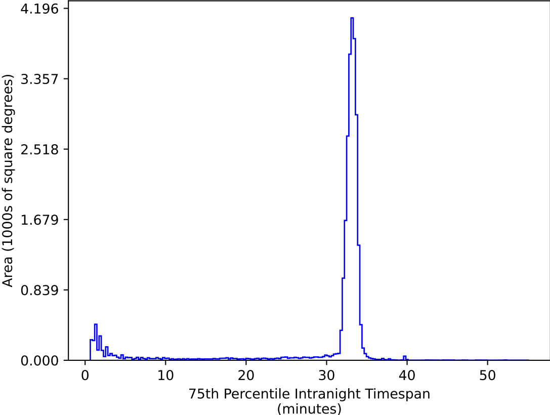
ddf_acor_sf30_lsf40_lsr10_v3.4_10yrs All sky ug bands: 75th Percentile Intranight Timespan
