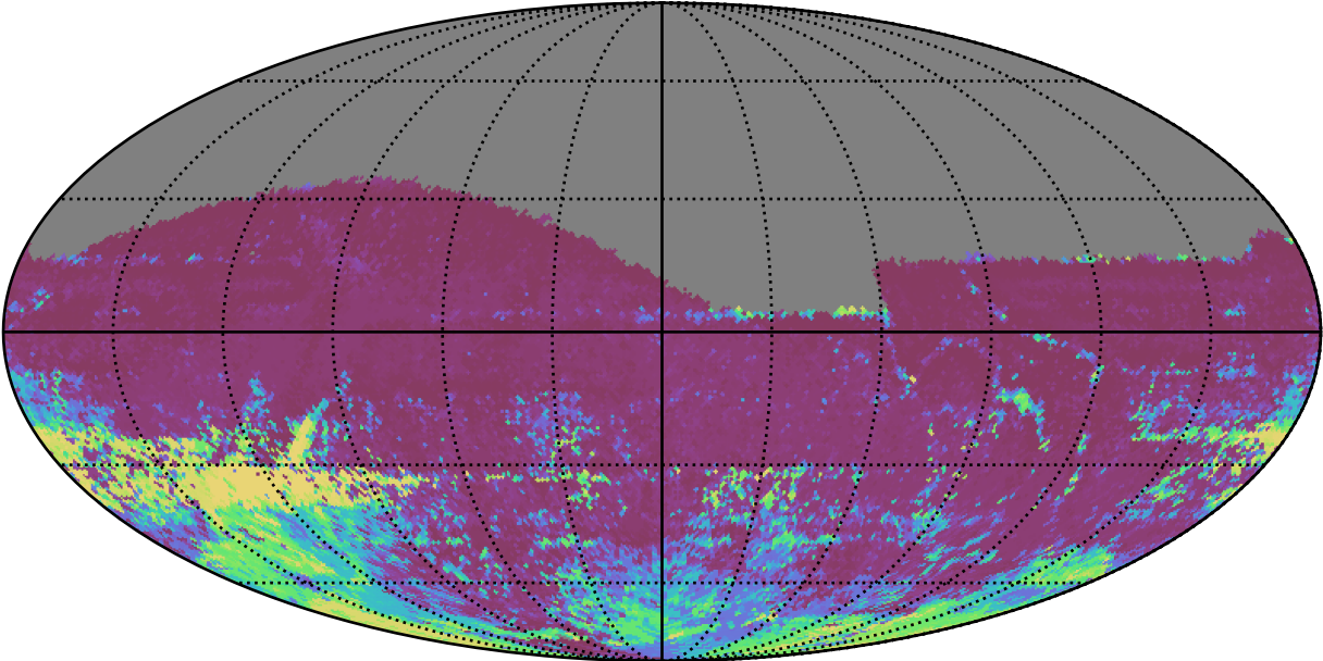
ddf_acor_sf30_lsf40_lsr10_v3.4_10yrs All sky r band: 75th Percentile Intranight Timespan
