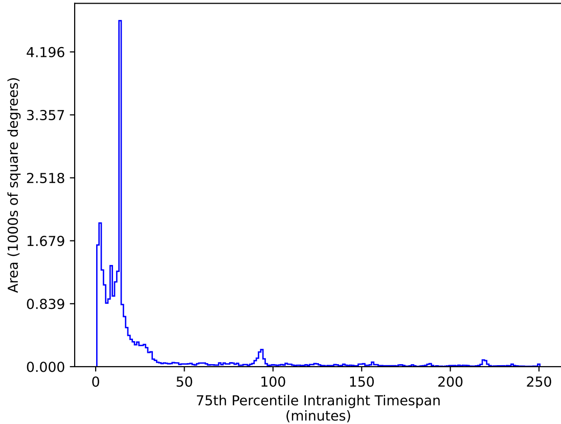
ddf_acor_sf30_lsf40_lsr10_v3.4_10yrs All sky i band: 75th Percentile Intranight Timespan
