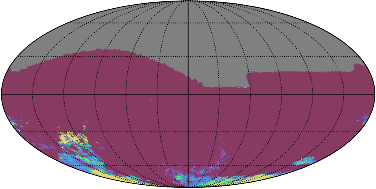
ddf_acor_sf30_lsf40_lsr10_v3.4_10yrs All sky gr bands: 75th Percentile Intranight Timespan
