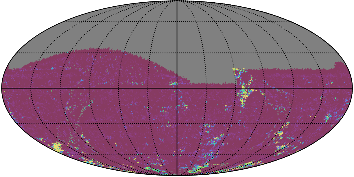
ddf_acor_sf30_lsf40_lsr10_v3.4_10yrs All sky g band: 75th Percentile Intranight Timespan
