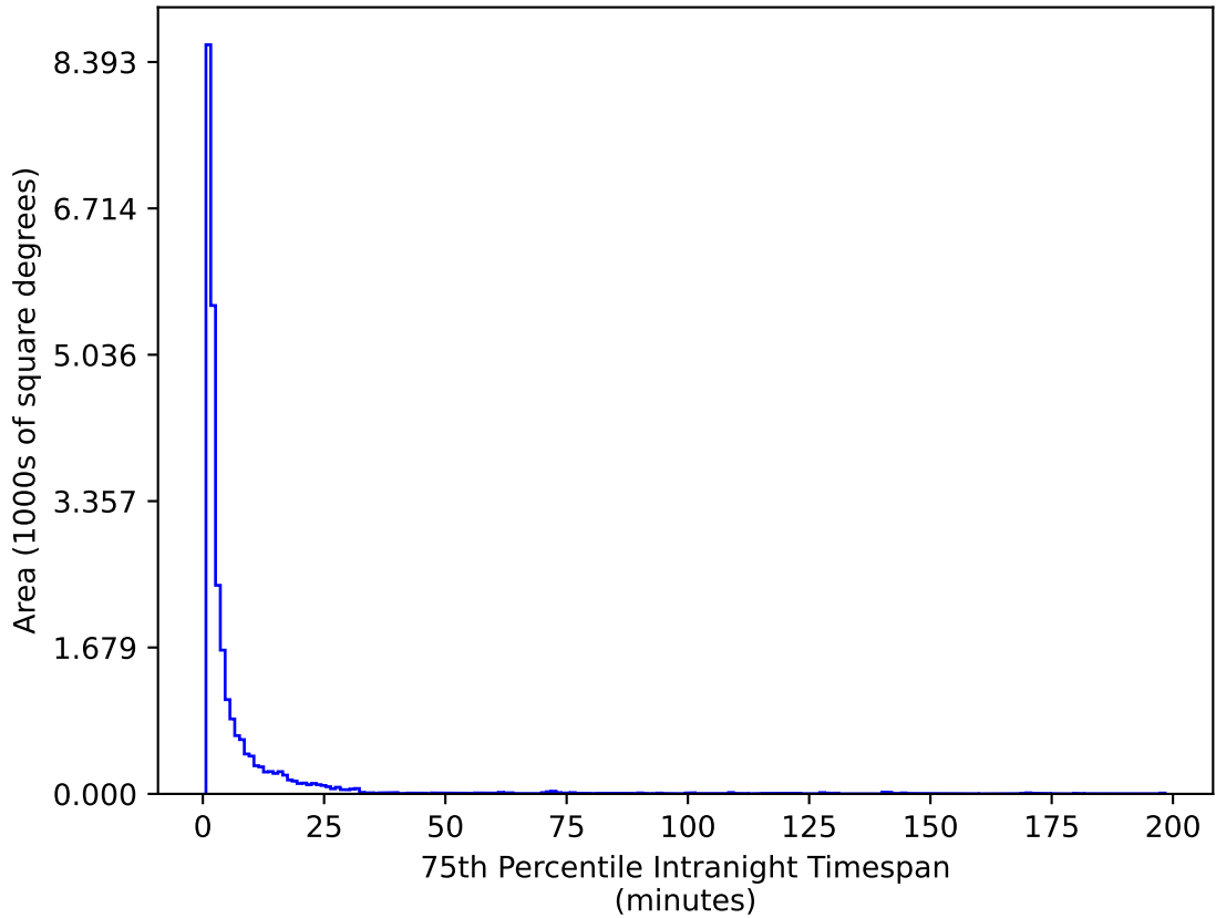
ddf_acor_sf30_lsf40_lsr10_v3.4_10yrs All sky g band: 75th Percentile Intranight Timespan
