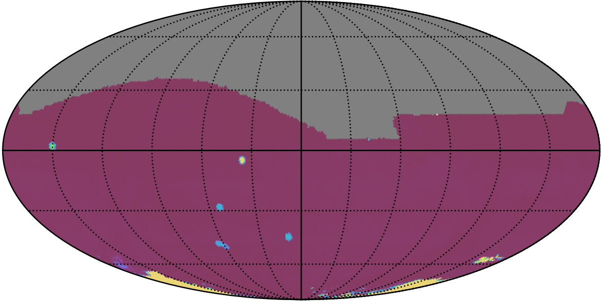
ddf_acor_sf30_lsf40_lsr10_v3.4_10yrs All sky all bands: 75th Percentile Intranight Timespan
