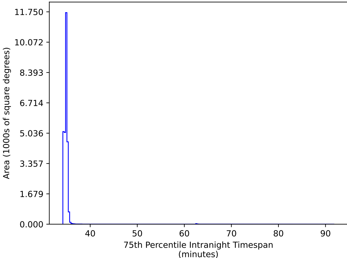
ddf_acor_sf30_lsf40_lsr10_v3.4_10yrs All sky all bands: 75th Percentile Intranight Timespan
