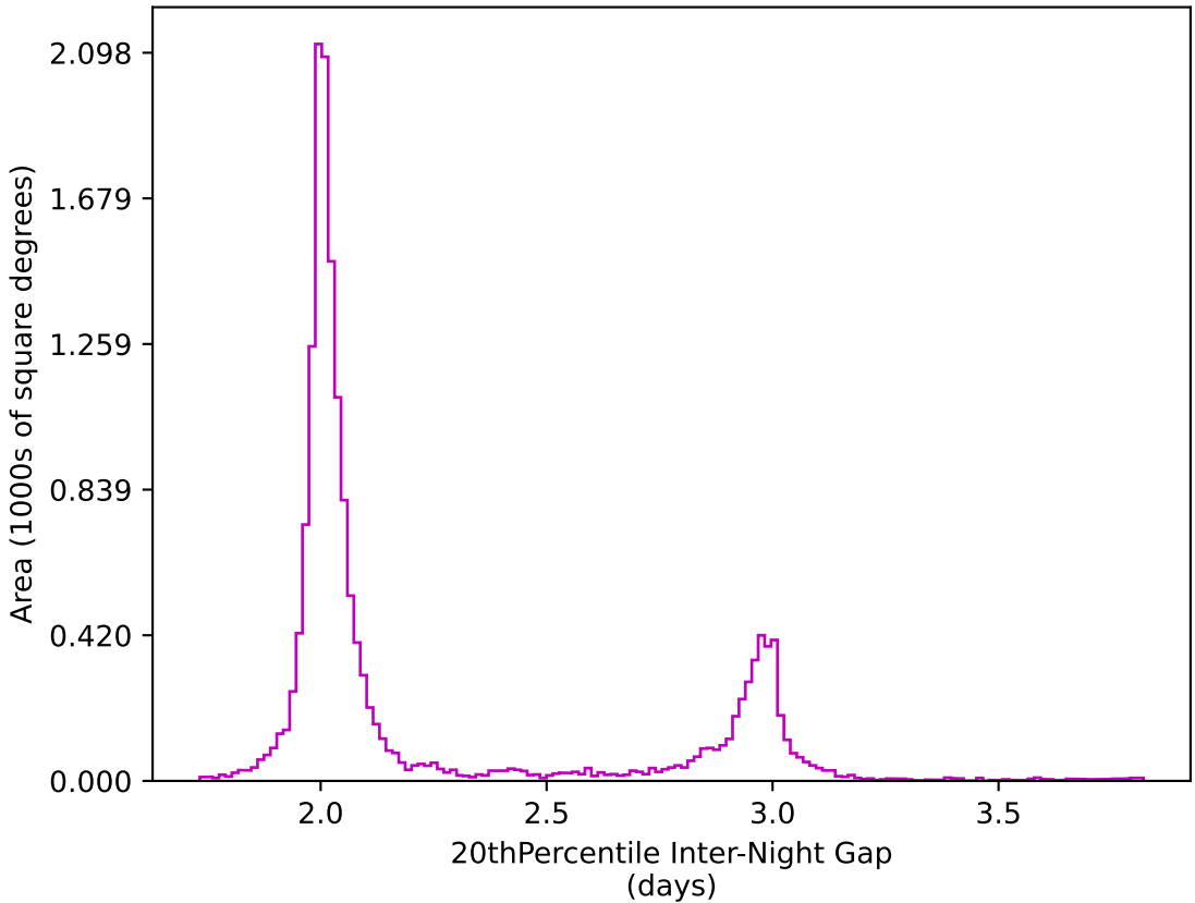
ddf_acor_sf30_lsf40_lsr10_v3.4_10yrs WFD z band: 20thPercentile Inter-Night Gap
